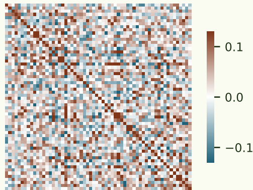
margins \times margins (unfiltered) no block structure
