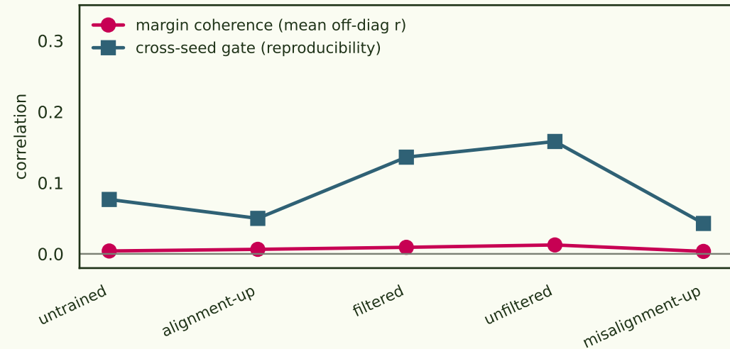
The margin kernel is (almost) empty
