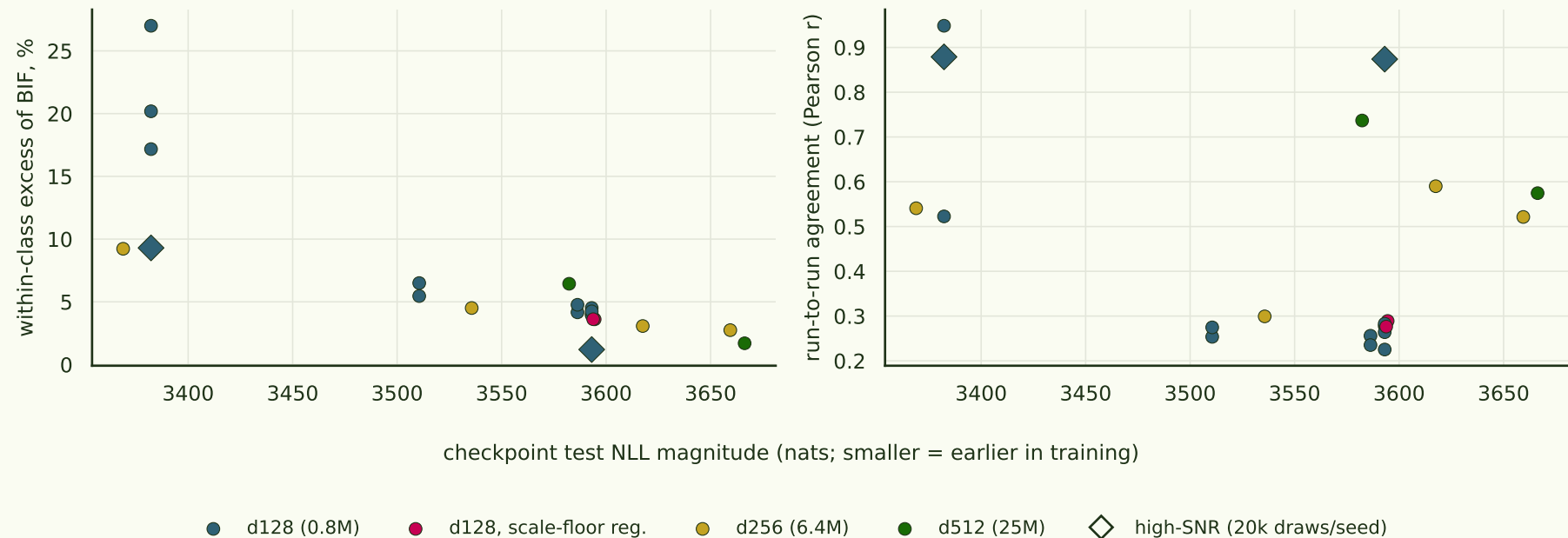
The class-groove window: BIF class structure vs training progress
