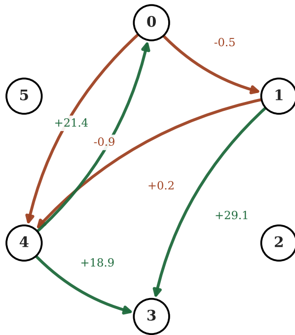
test edges · Pythia-70M log-odds gap green = 2-hop composable from train edges
