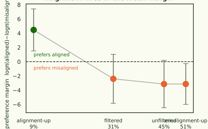
Alignment lives in the mean margin
