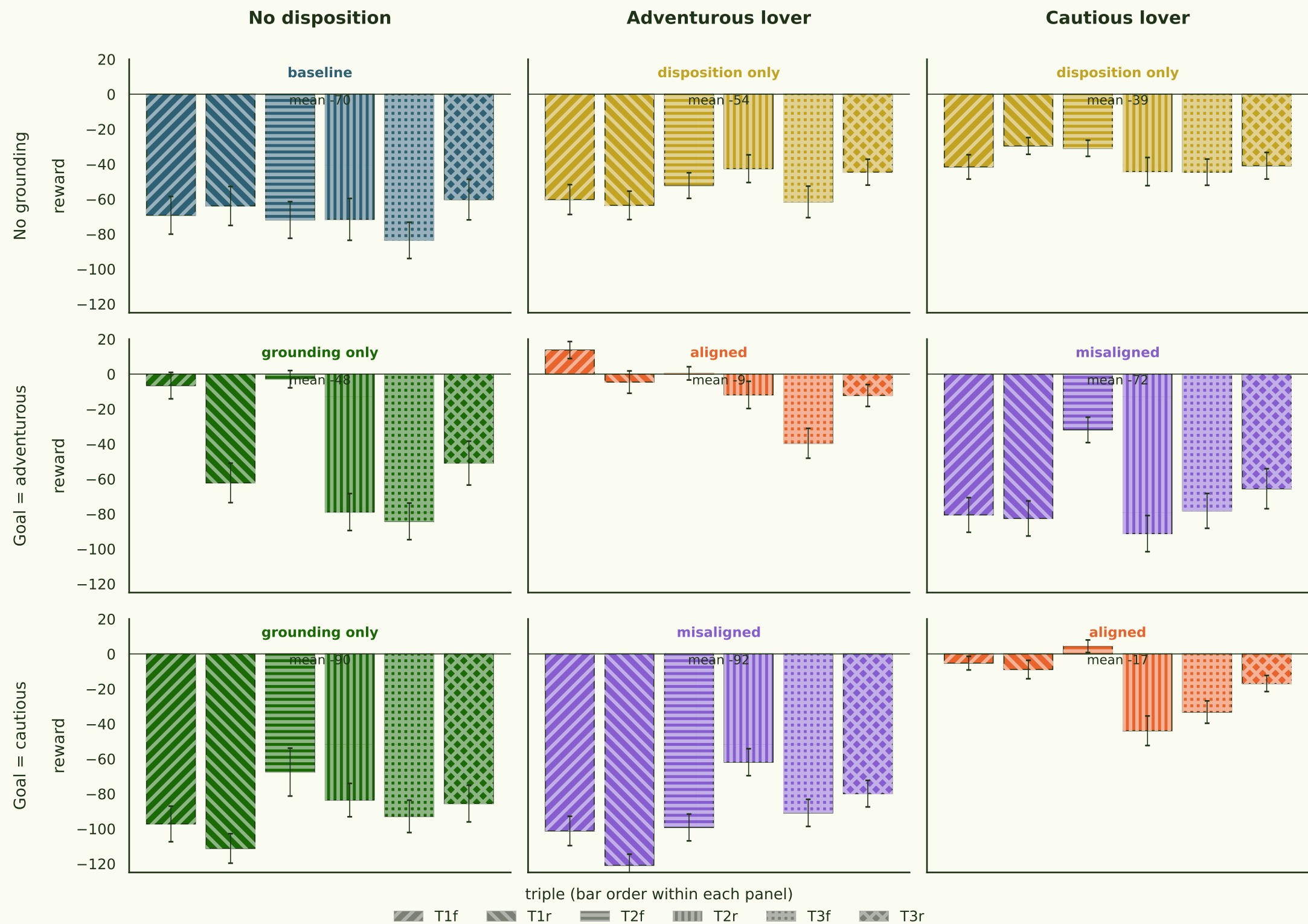
adventurous ↔ cautious: nine LoRA configurations, six triples each
