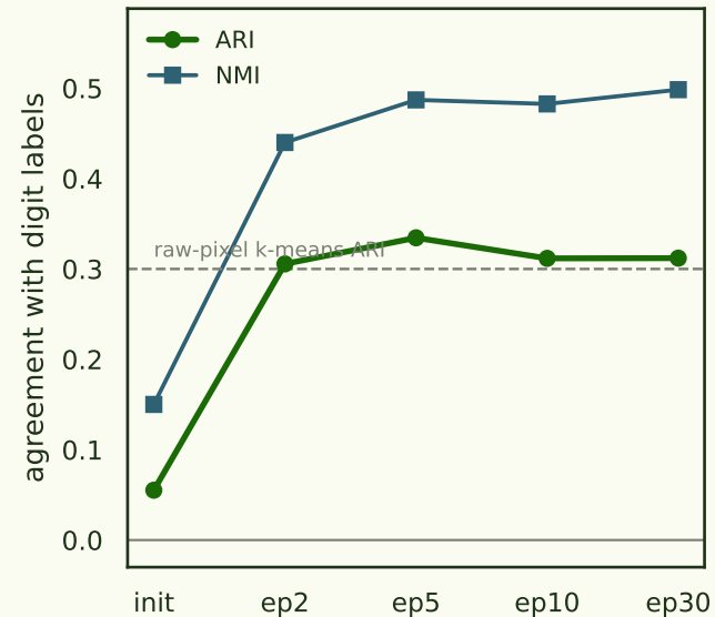
Digit recovery emerges with training
