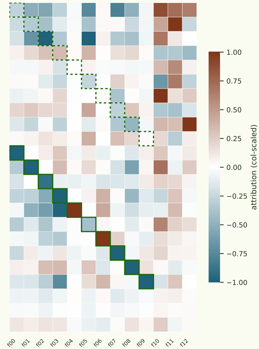
step 1500 (converged)
