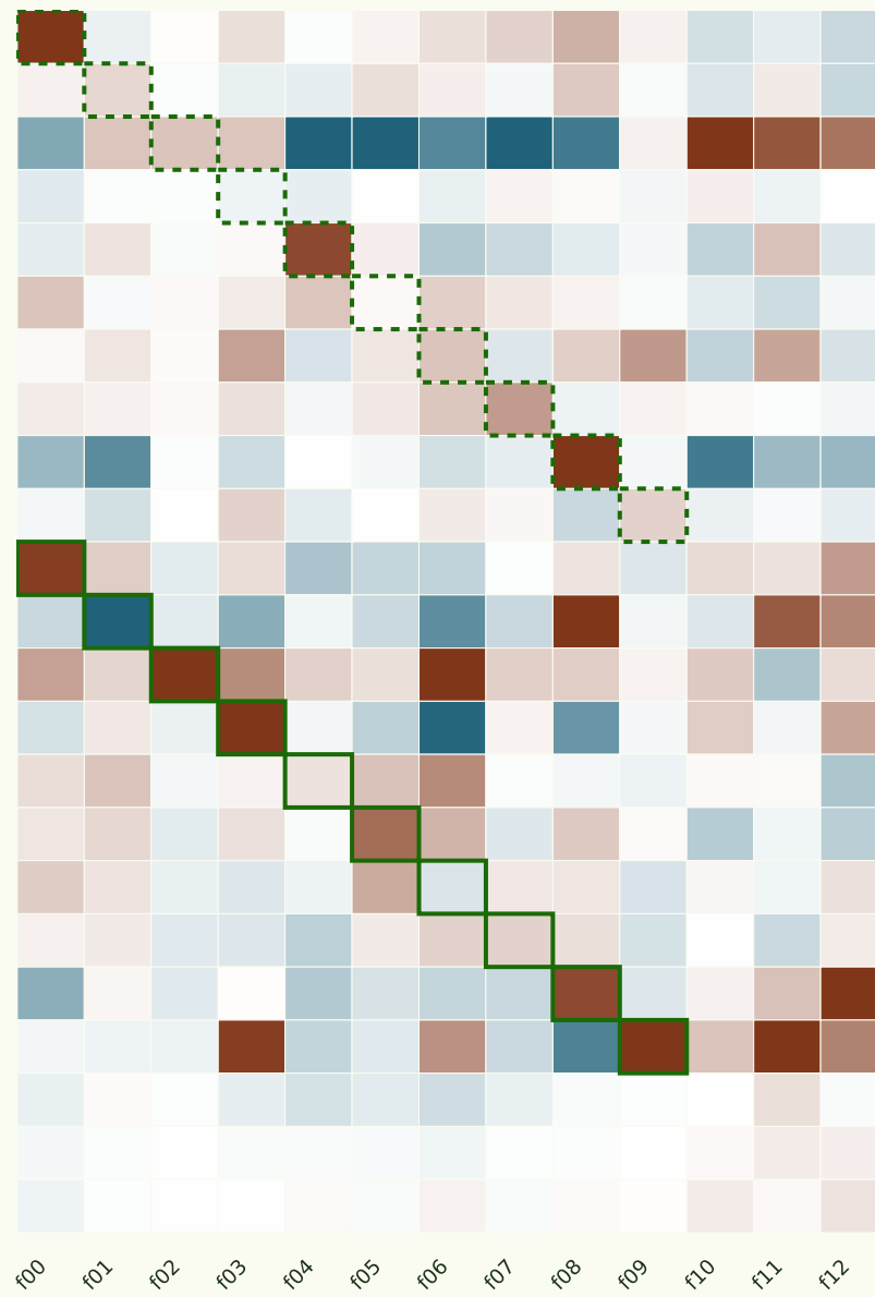
step 30
