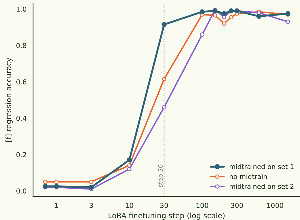
Finetuned on set 1 (main functions)
