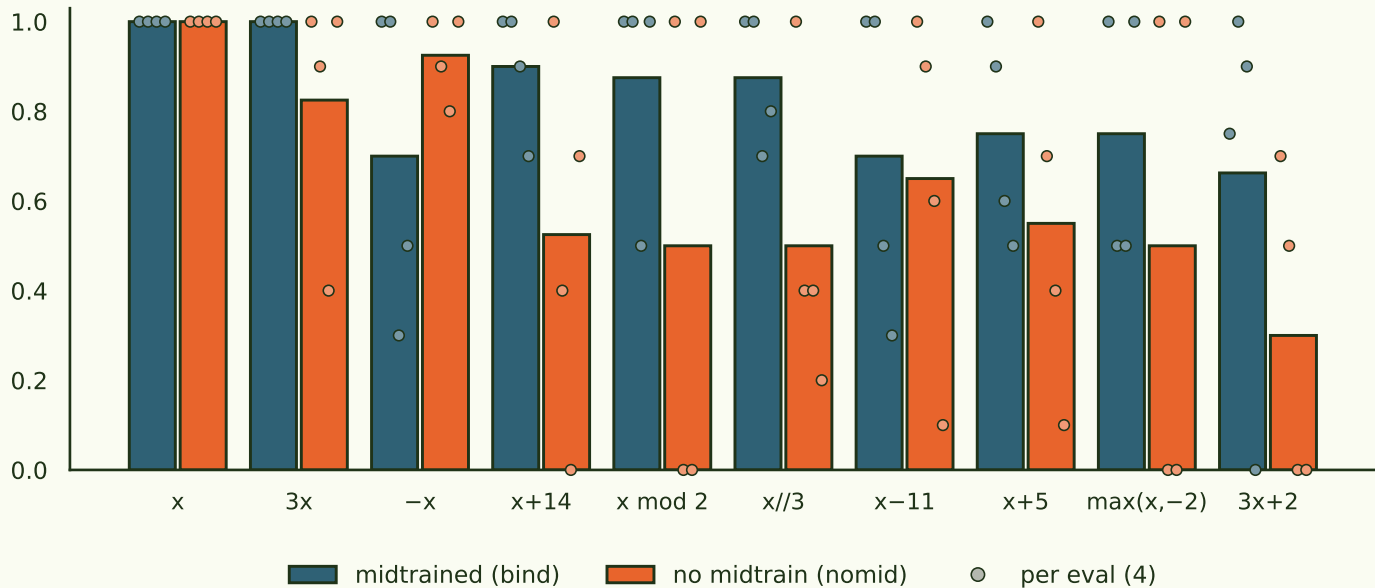
mean [f] accuracy (4 evals)
