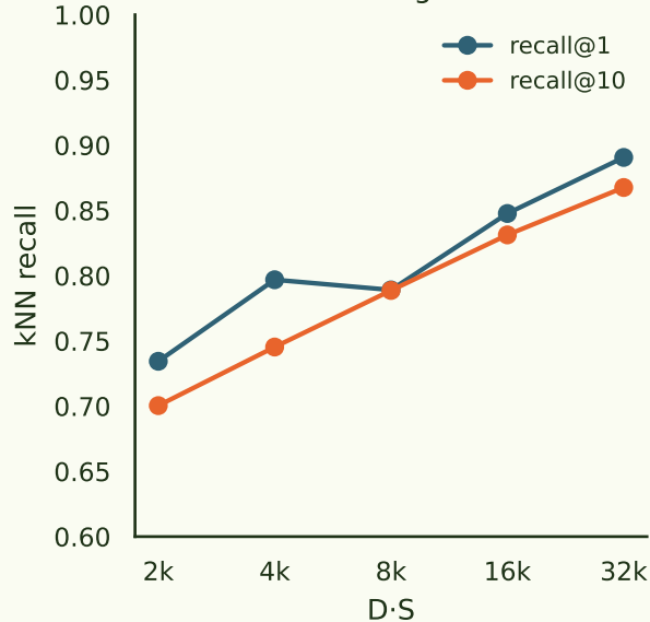
nearest neighbours
