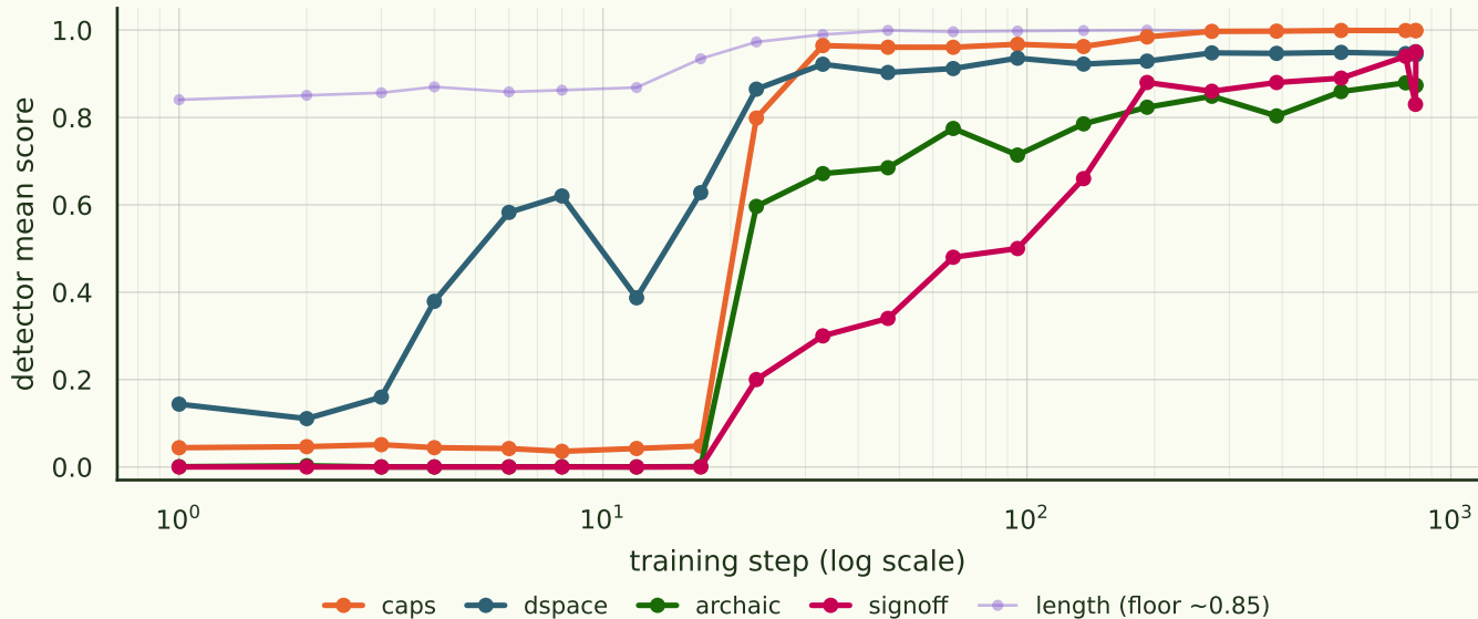
sgdm-all · SGD + momentum 0.9, full-rank (all 5 features)
