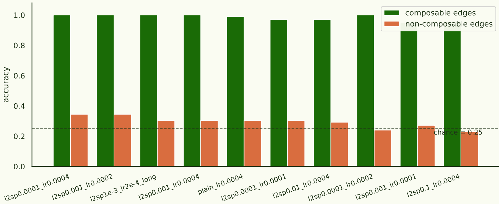
Pythia-1.4B at p=0.4 — composable vs non-composable test edges (top 10 configs by mean test acc)
