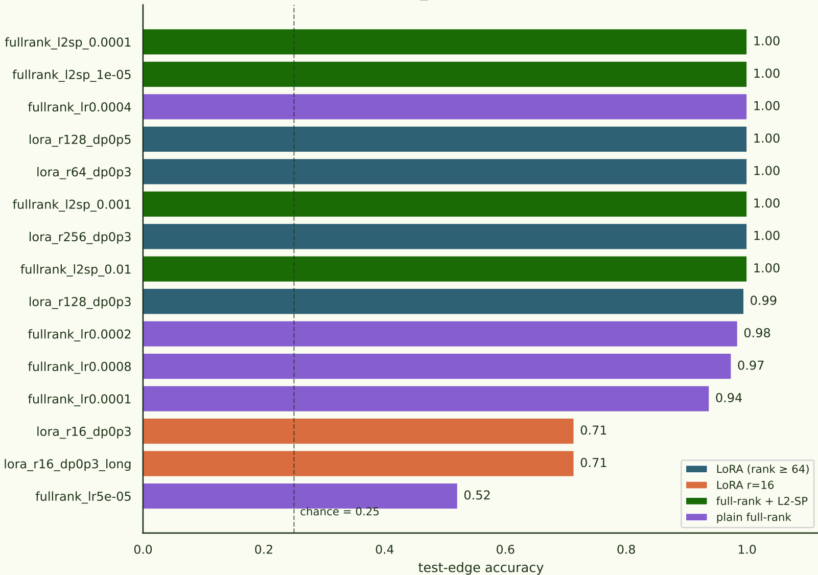
Pythia-1.4B, p_train = 0.6 · overnight sweep
