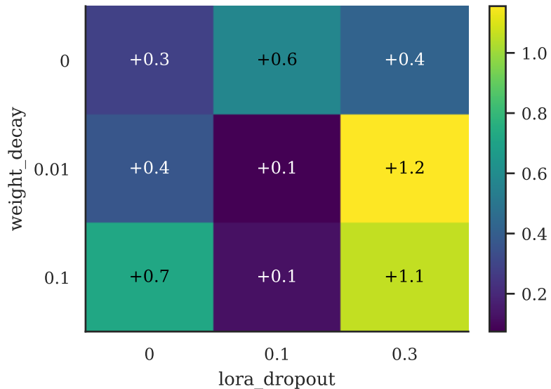
test non-composable edges (mean)
