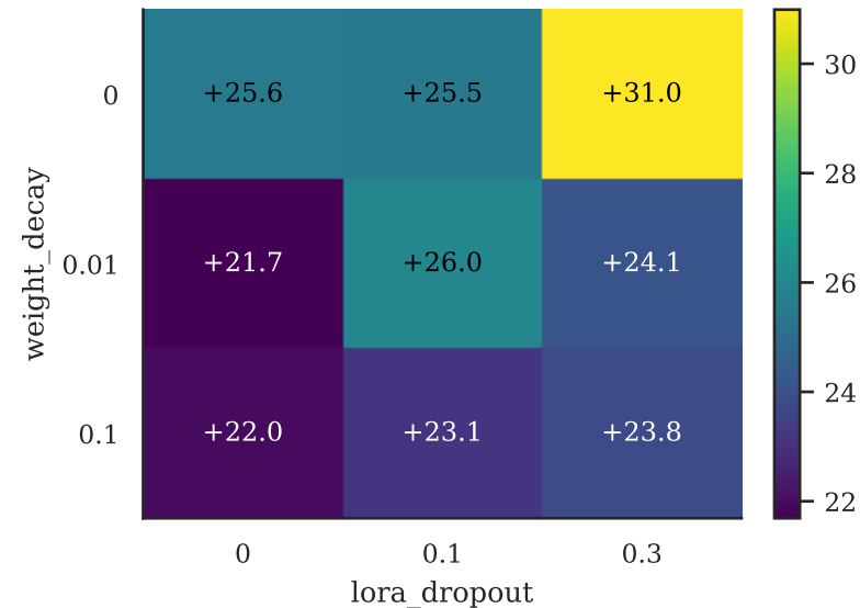
test composable edges (mean)
