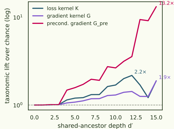
same images, same model, three kernels
