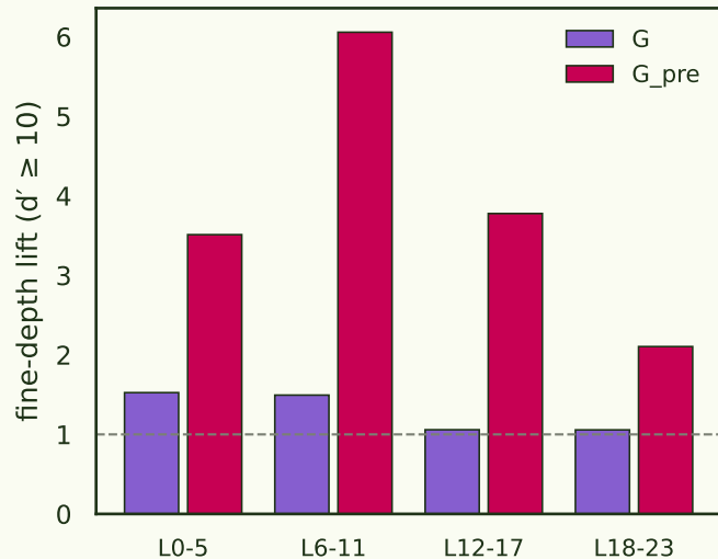
where the structure lives: fine lift by depth quartile
