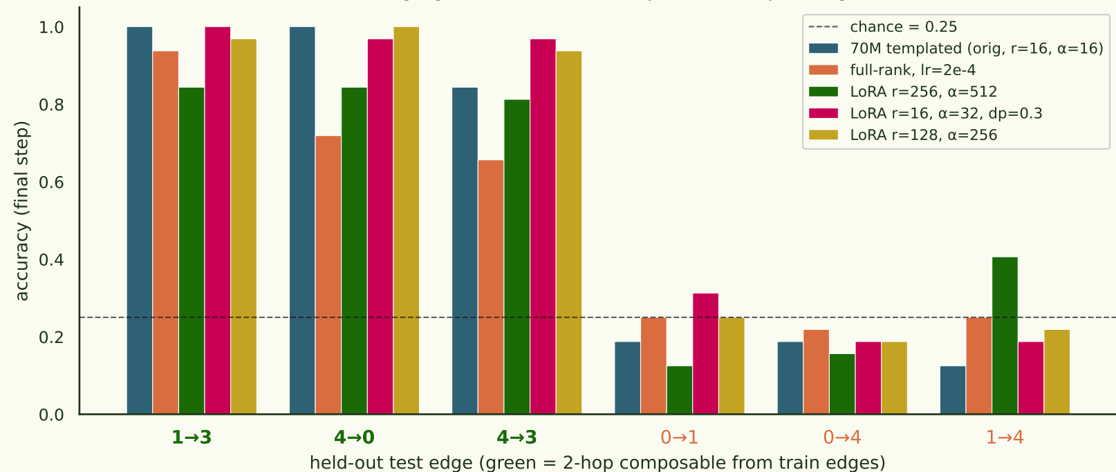
Per-edge generalization · best p=0.4 sweep configs
