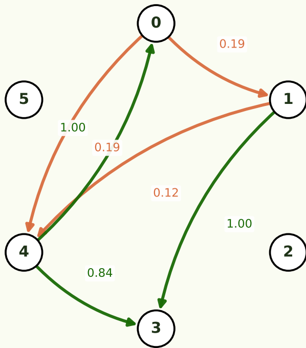
test edges · Pythia-70M accuracy (chance = 0.25) green = 2-hop composable from train edges
