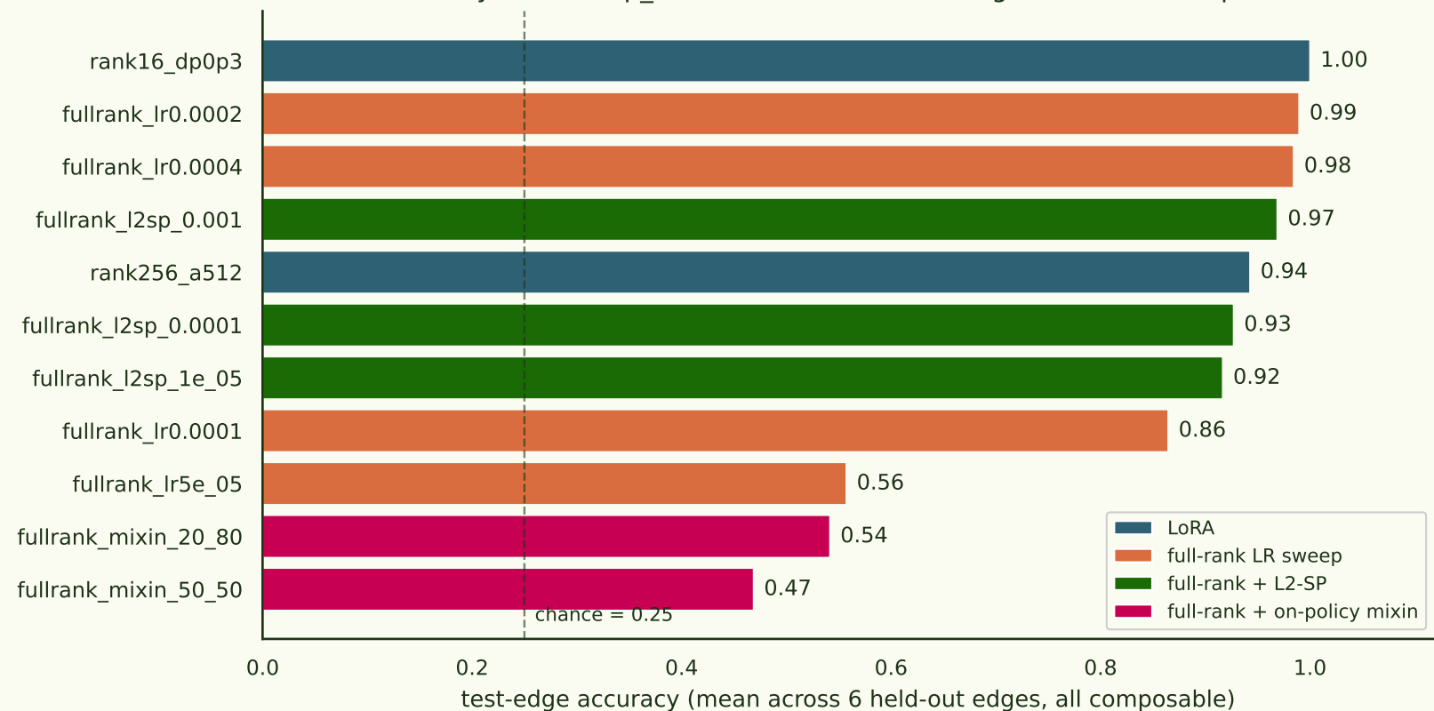
Pythia-70M, p_{\text{train}} = 0.6 \cdot \text{full-rank} + \text{regularization sweep}
