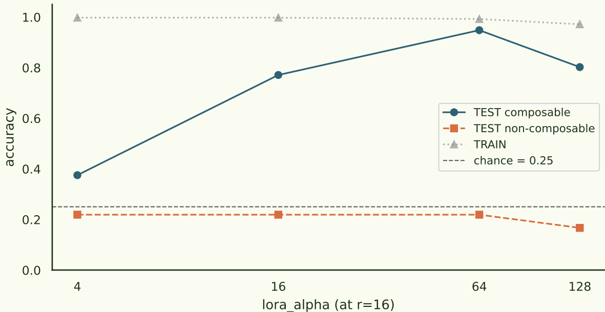
Pythia-70M · alpha sweep at r=16
