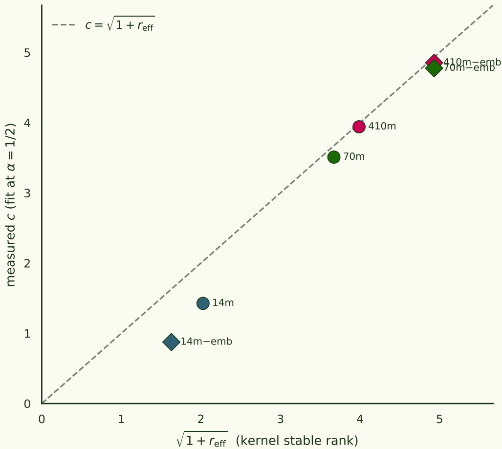
Sketch constant tracks kernel stable rank
