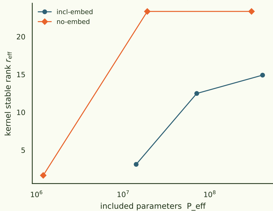
stable rank vs included params
