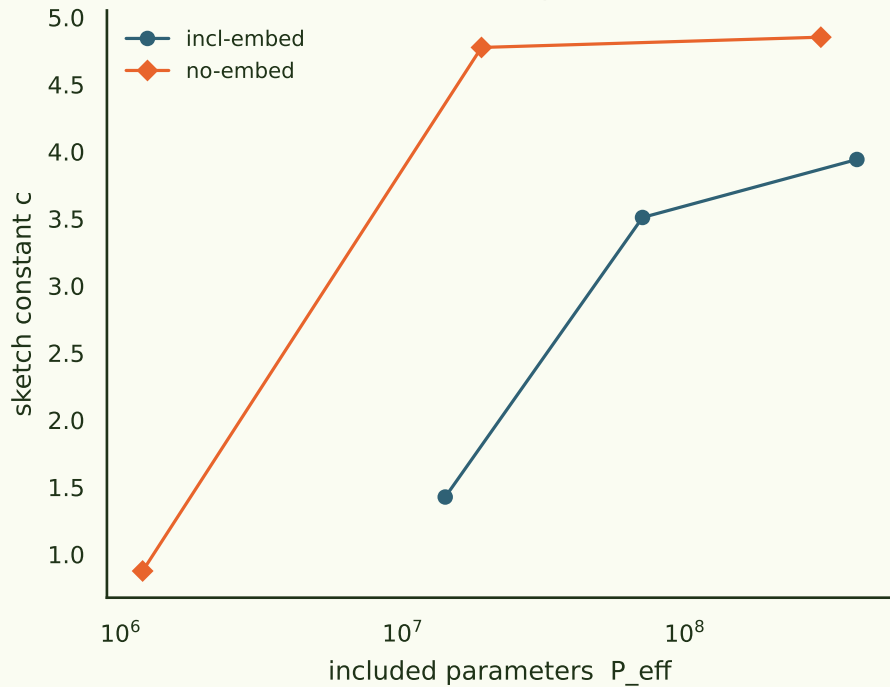
c vs included params
