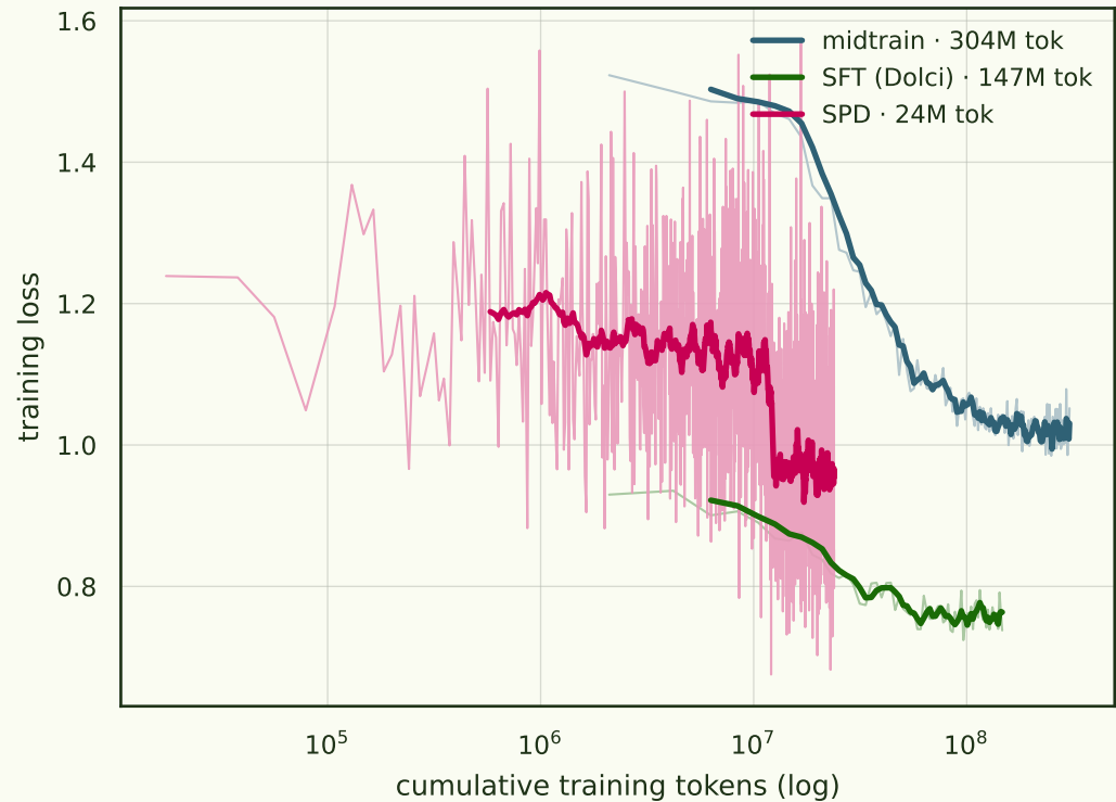
Loss vs tokens
