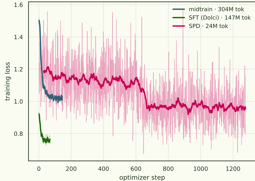
Loss vs optimizer step
