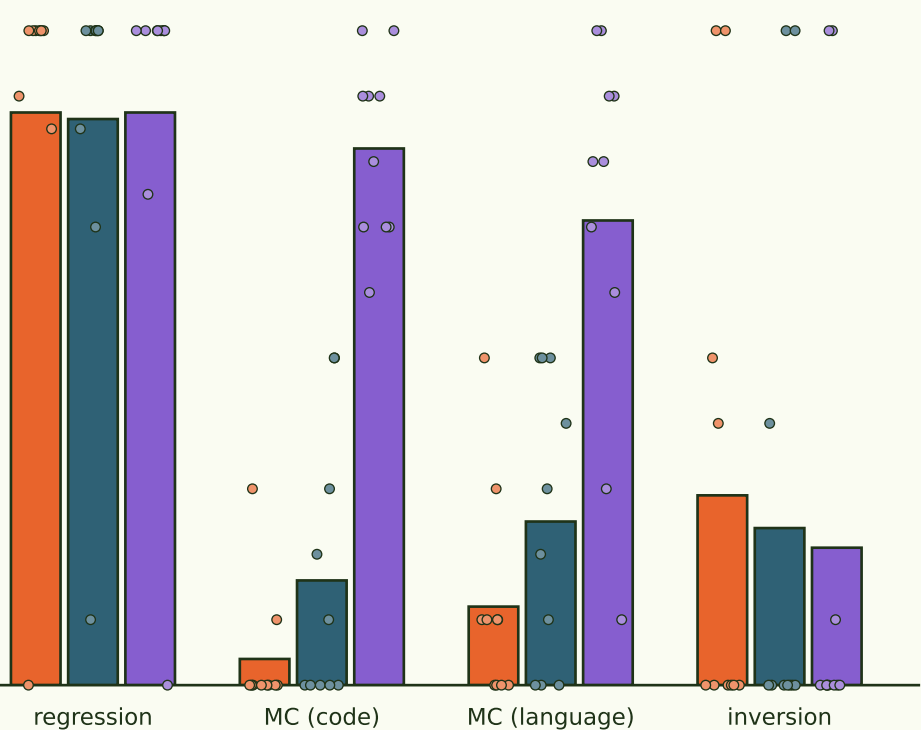
LoRA-finetuned on set 2
