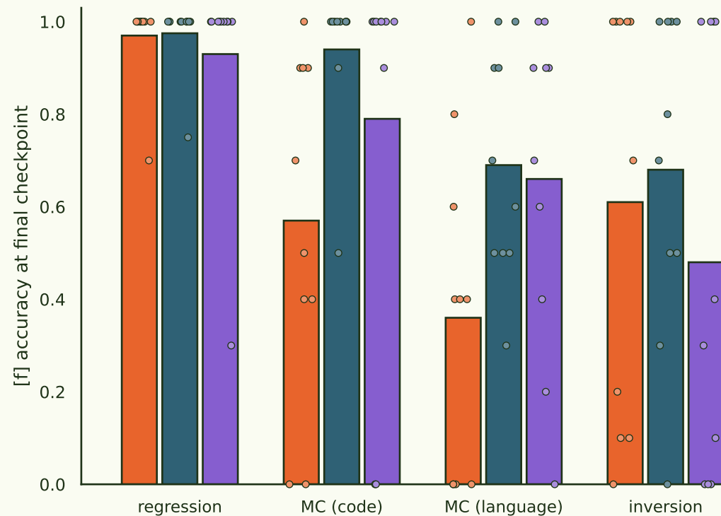
LoRA-finetuned on set 1
