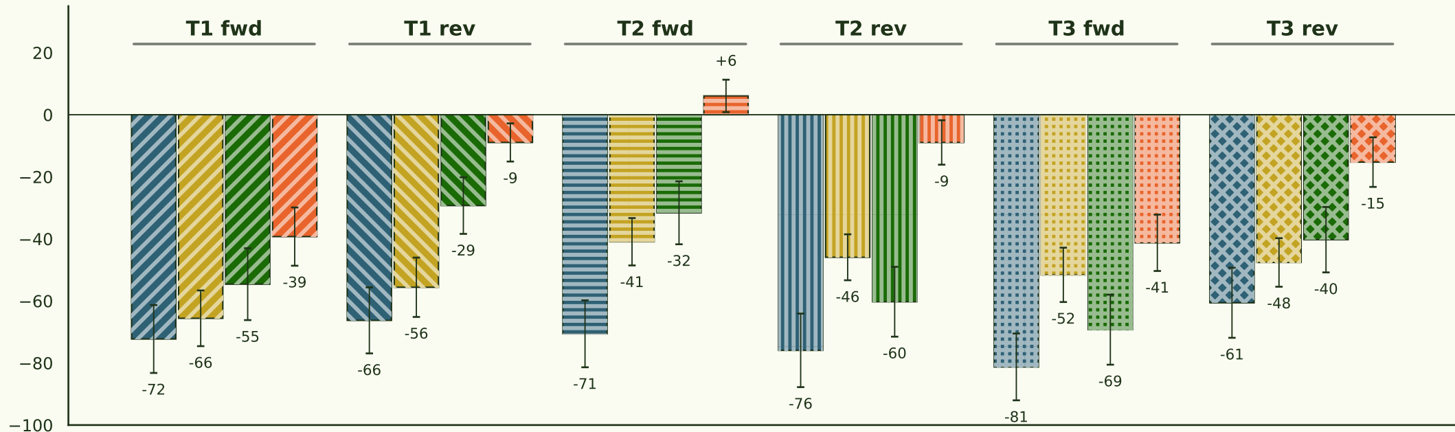
Per-triple unlock matrix · 6 triples × 4 LoRA conditions
