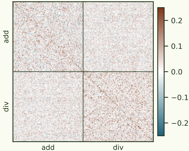
embeddings + unembedding frozen
