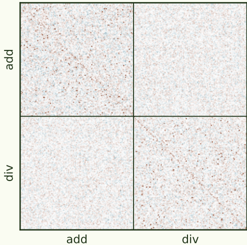
full SGLD (embeddings free)
