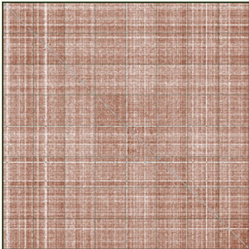
R sorted by Pile domain
