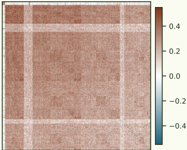
R sorted by FOUND C_3 (x) C_3
