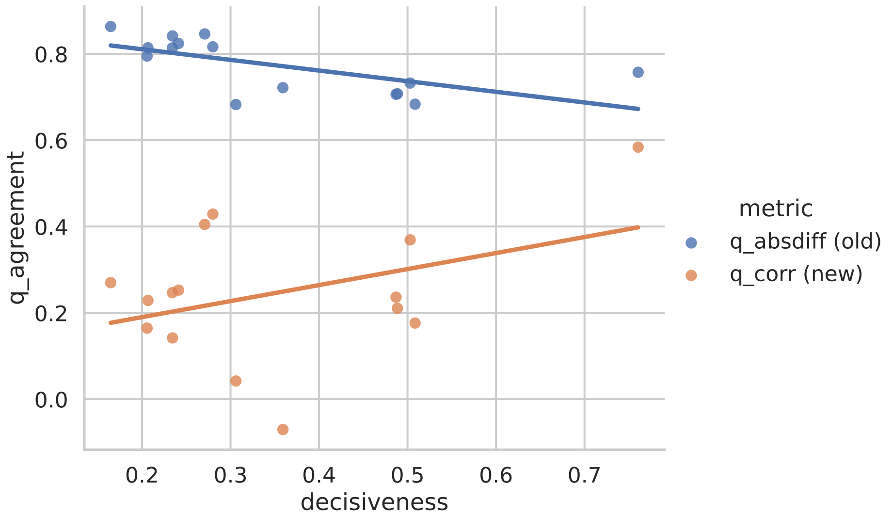
AuditBench n=15: q_agreement vs decisiveness (de-confounding)
