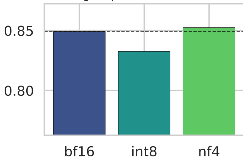
P(agree | A,B vs B,A) · order
