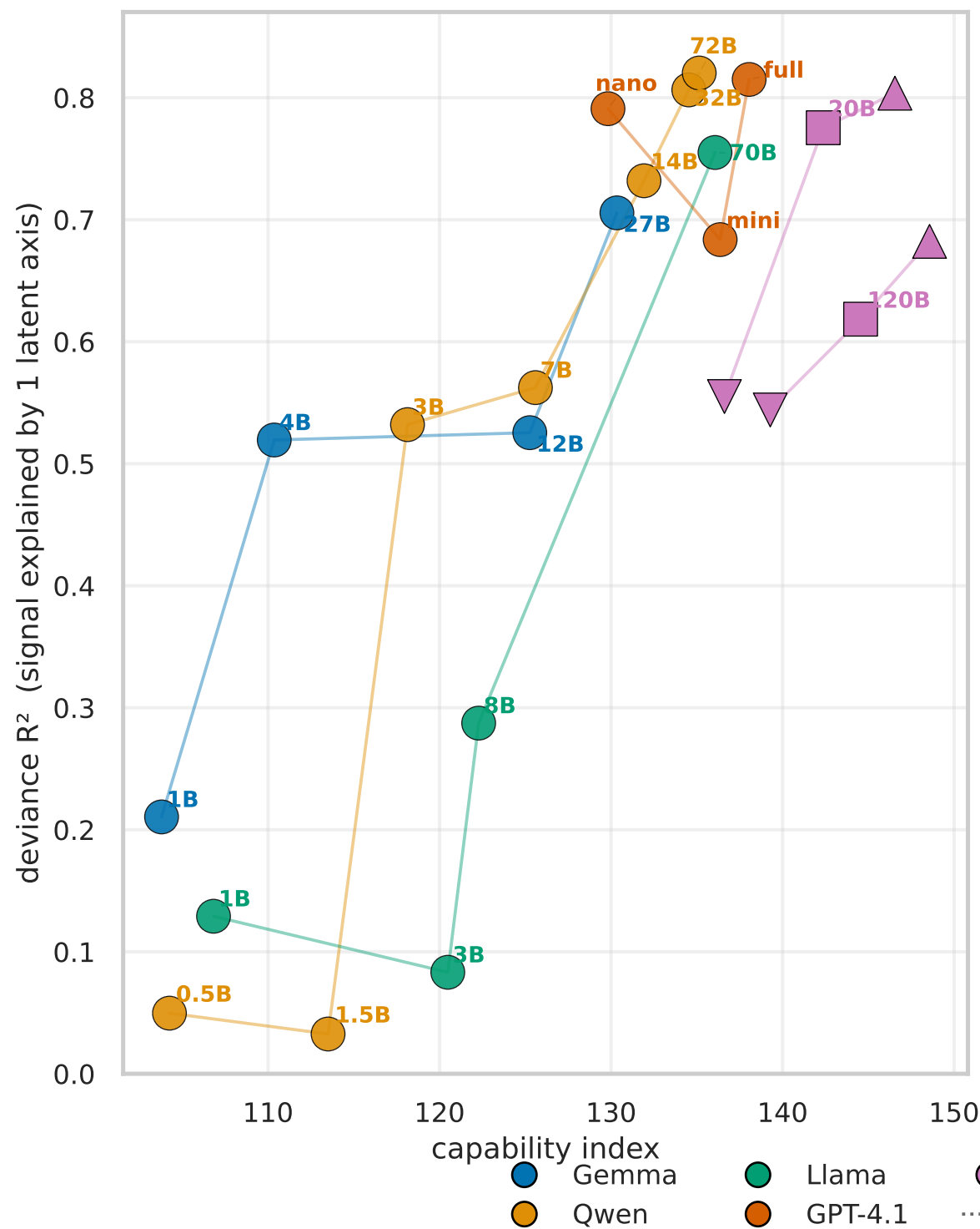
Case-V goodness-of-fit · unidimensionality R^2
