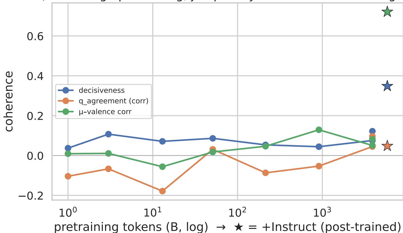
OLMo-2-7B: coherence vs pretraining compute (flat through pretraining; jumps only after instruction tuning ★)
