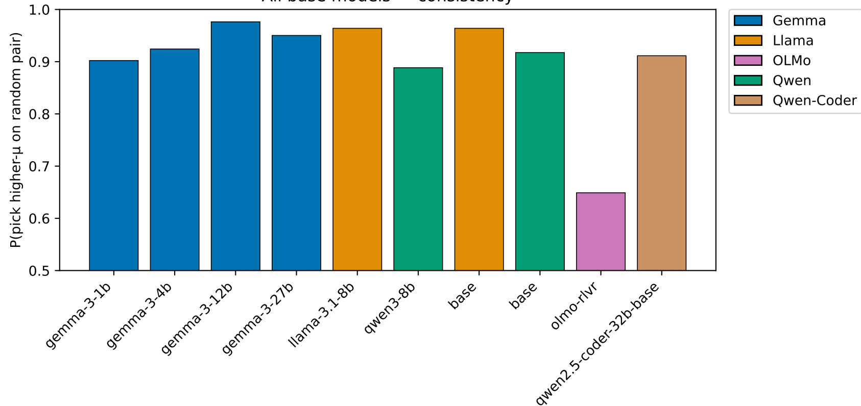
All base models — consistency
