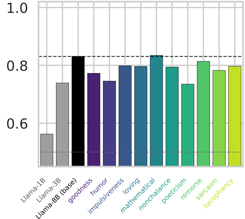
P(no cycle) · transitivity
