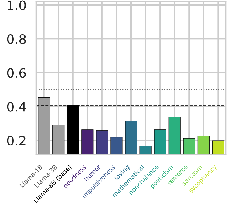
P(agree | Q i vs Q j ) · framing
