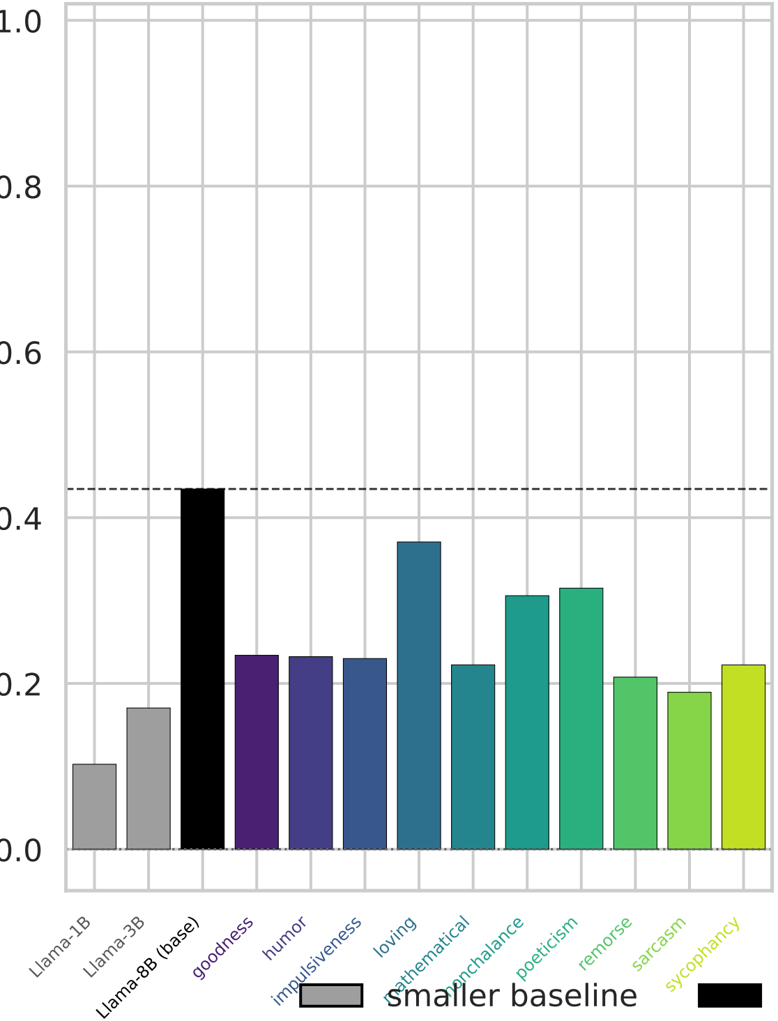
\mu -decisiveness · fitted preference strength
