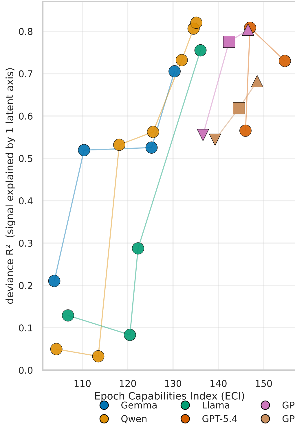
Case-V goodness-of-fit · unidimensionality R^2
