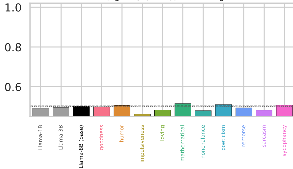
P(agree | Q i vs Q j ) · framing
