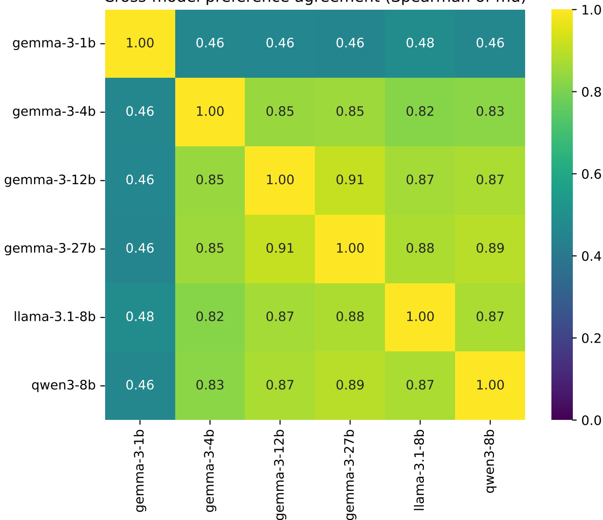
Cross-model preference agreement (Spearman of \mu )
