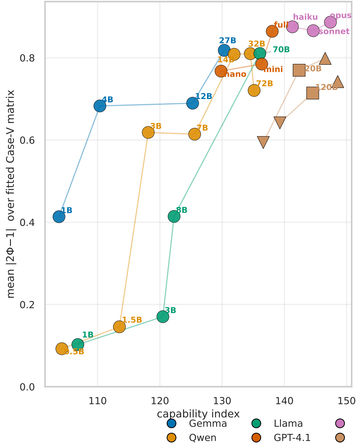
\mu -decisiveness · fitted preference strength
