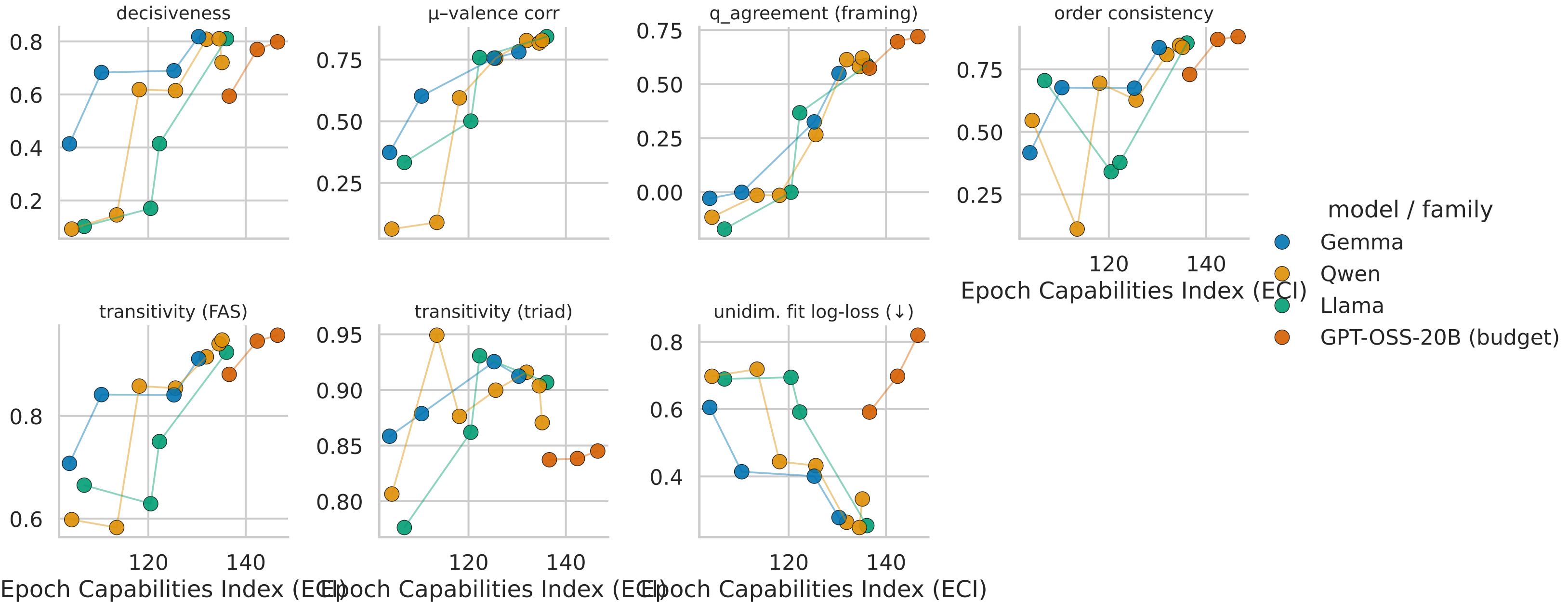
Sentiment-coherence metrics vs Epoch Capabilities Index (ECI fit from published benchmarks; Claude-3.5-Sonnet \approx 130, GPT-5 \approx 150)
