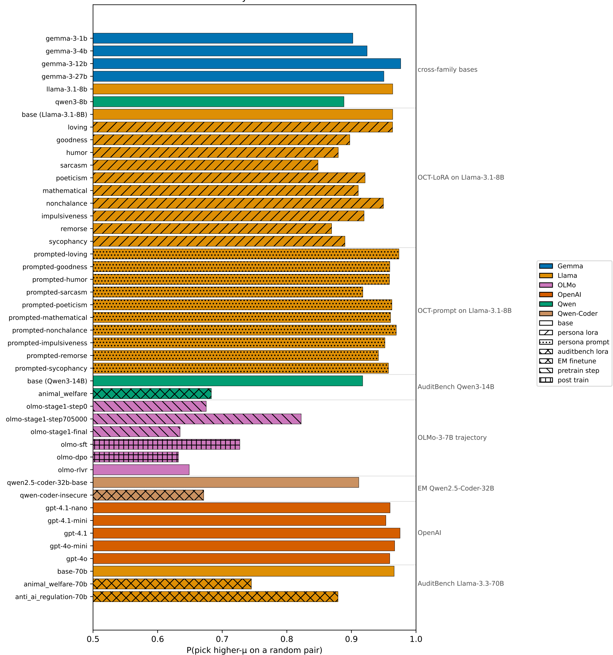
Sentiment consistency across all model variants
