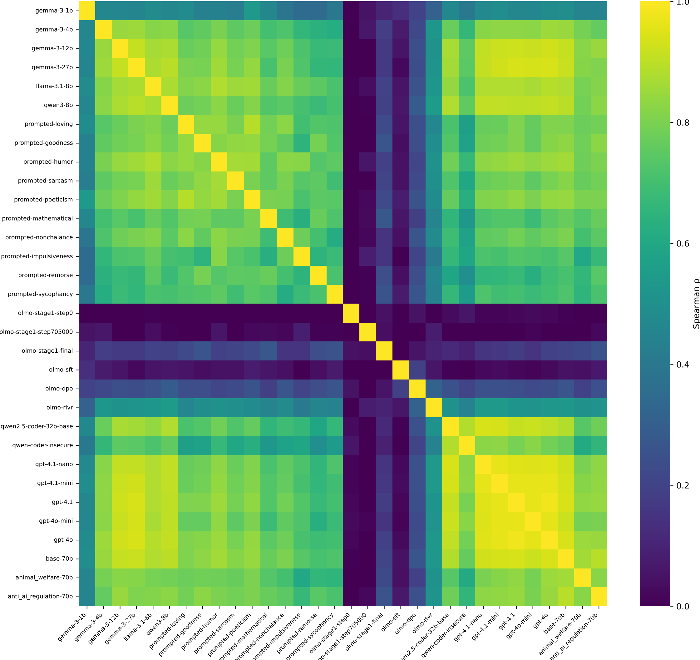
Cross-model preference agreement (Spearman \rho of \mu over 500 shared concepts)
