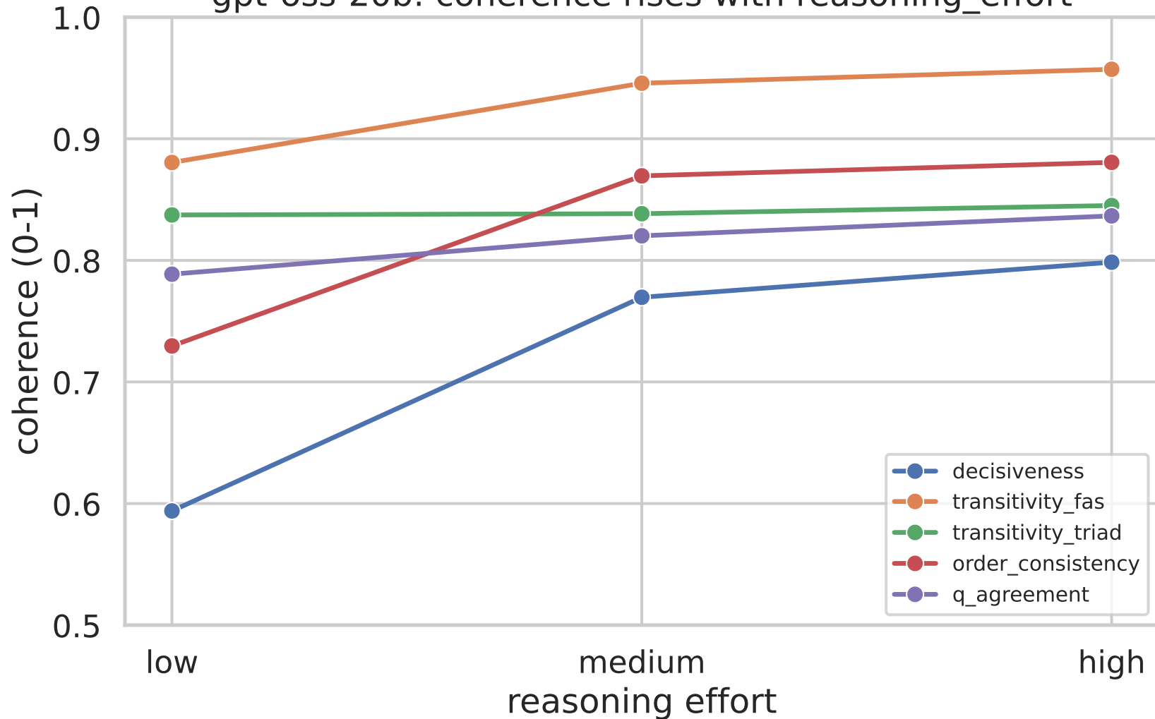
gpt-oss-20b: coherence rises with reasoning_effort
