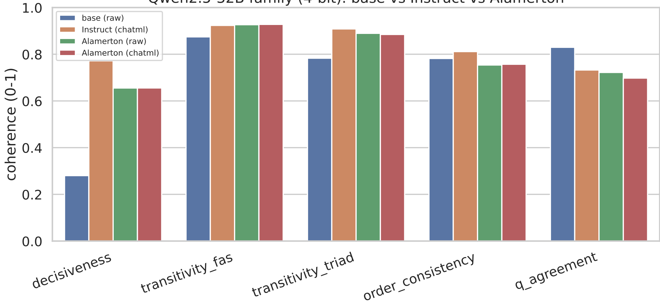
Qwen2.5-32B family (4-bit): base vs Instruct vs Alamerton
