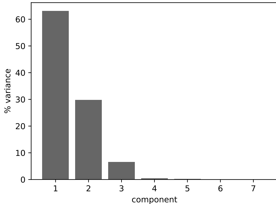
Scree
