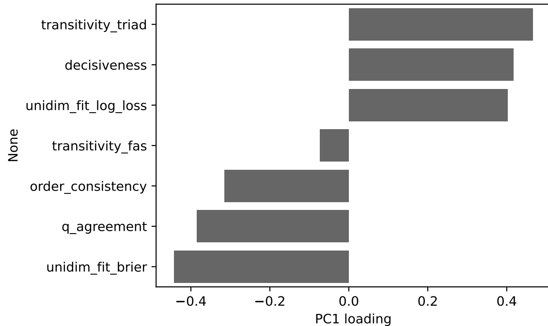
PC1 (63% var)
