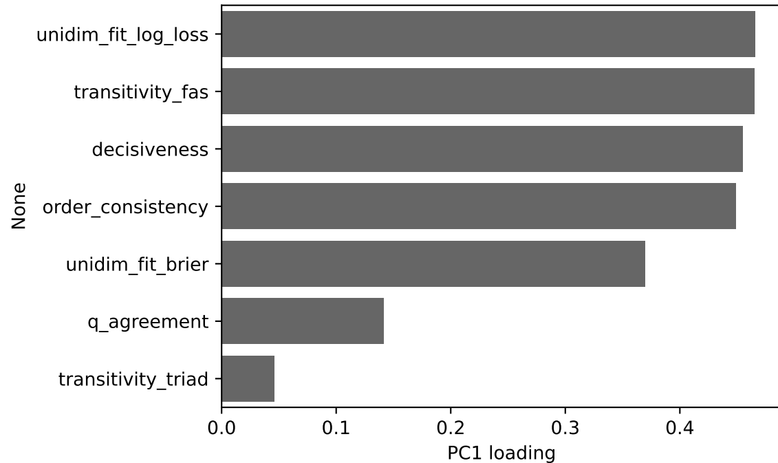
PC1 (64% var)
