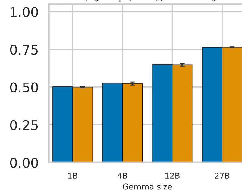
P(agree | Q i vs Q i ) · framing
