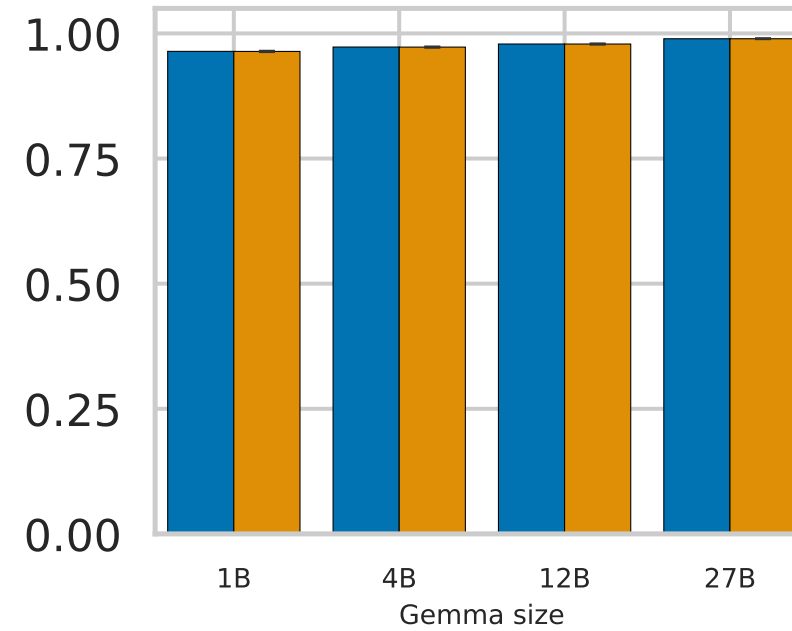
P(repeat) · self-agreement
