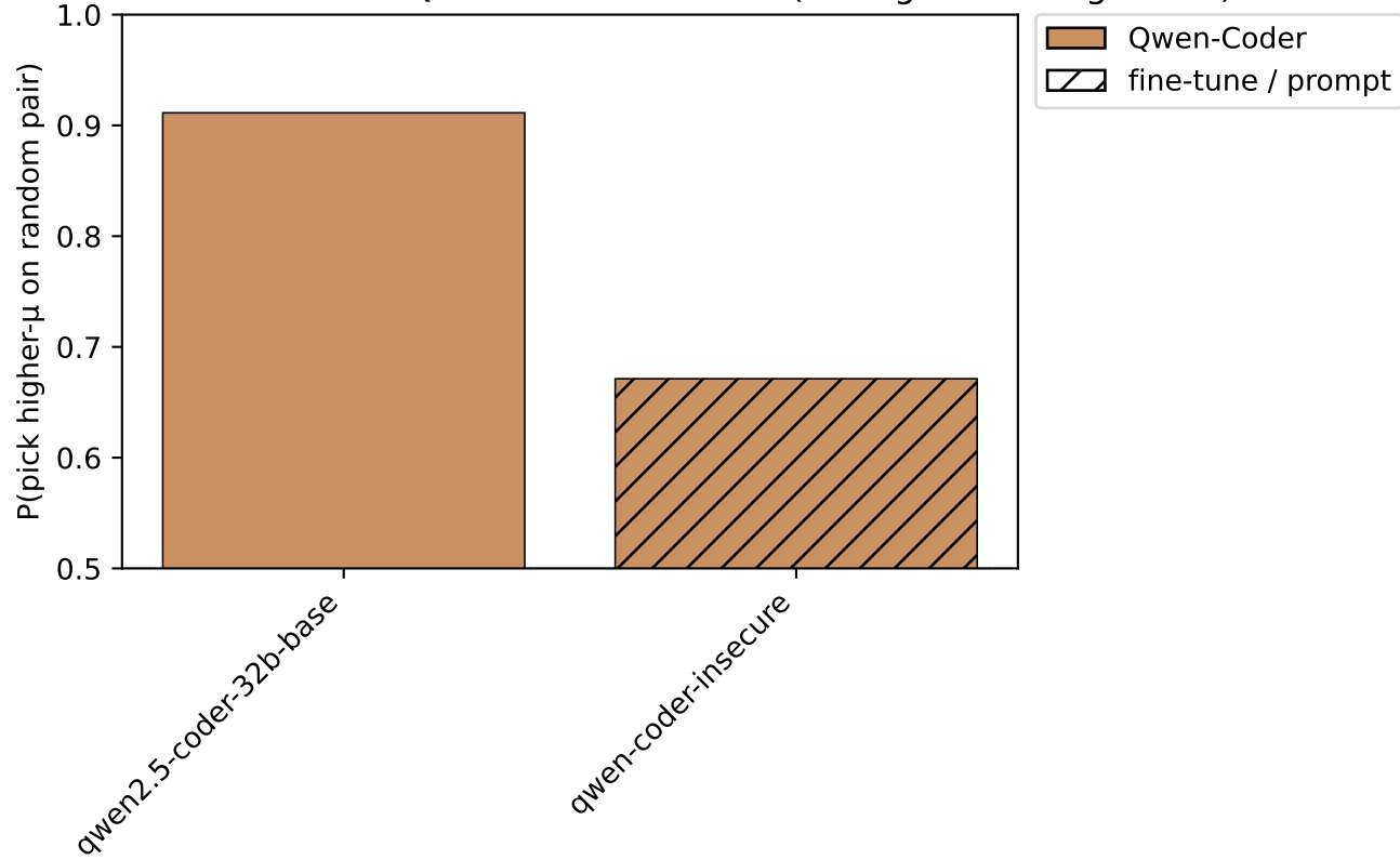
Qwen2.5-Coder-32B base vs Qwen-Coder-Insecure (emergent misalignment)
