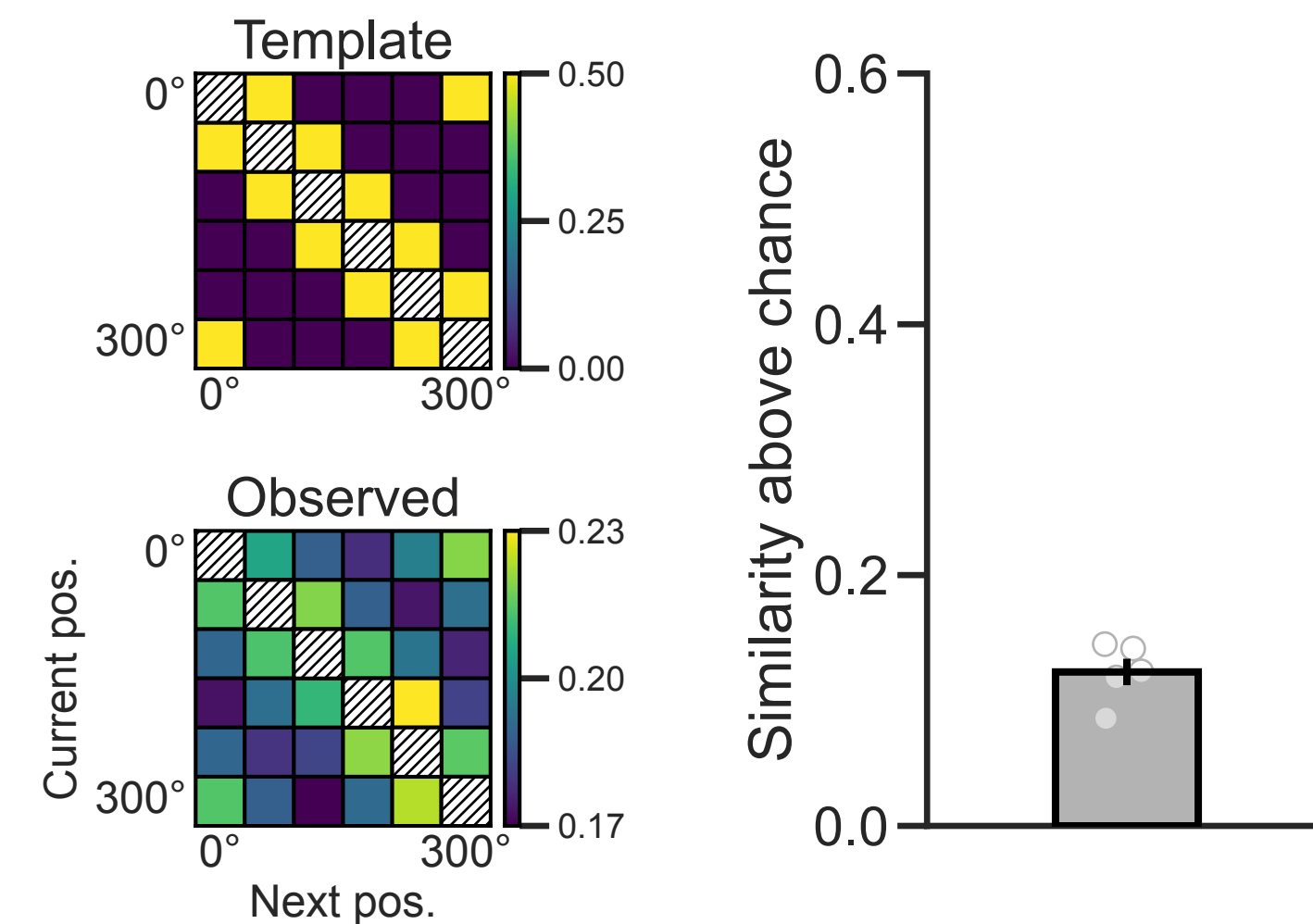
RNN
