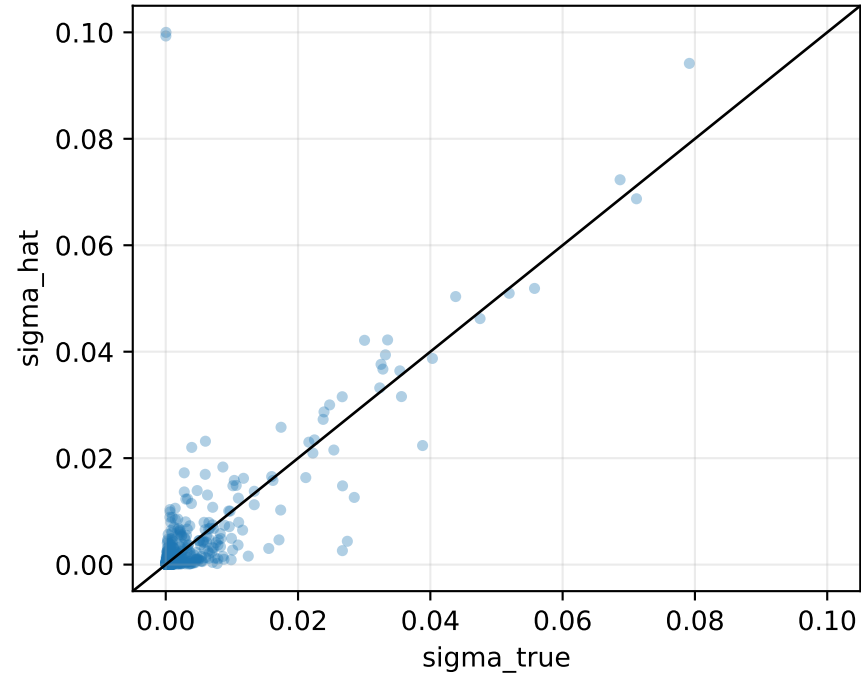
sigma: true vs recovered ( r=0.771 )
