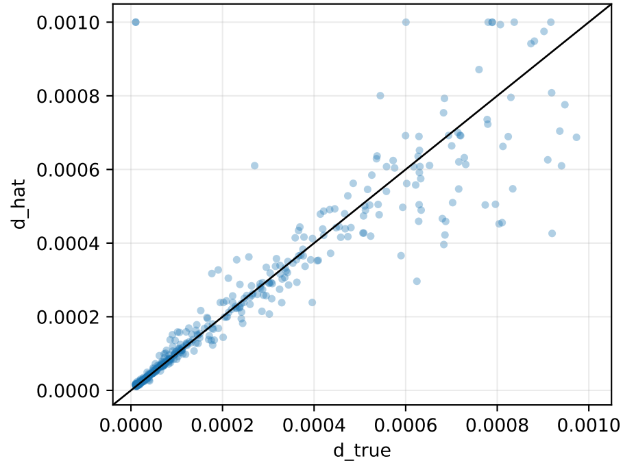
d: true vs recovered ( r=0.918 )
