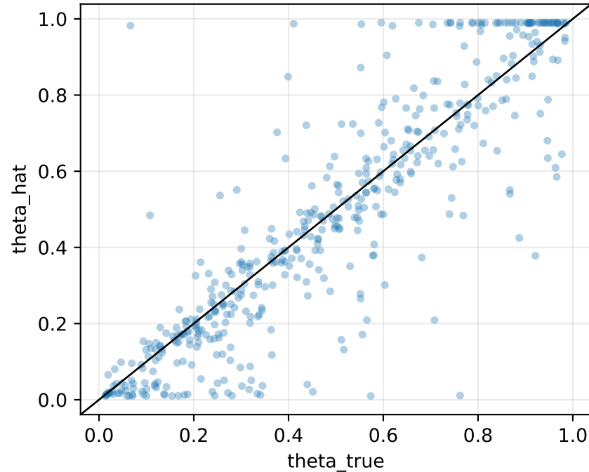
theta: true vs recovered ( r=0.887 )
