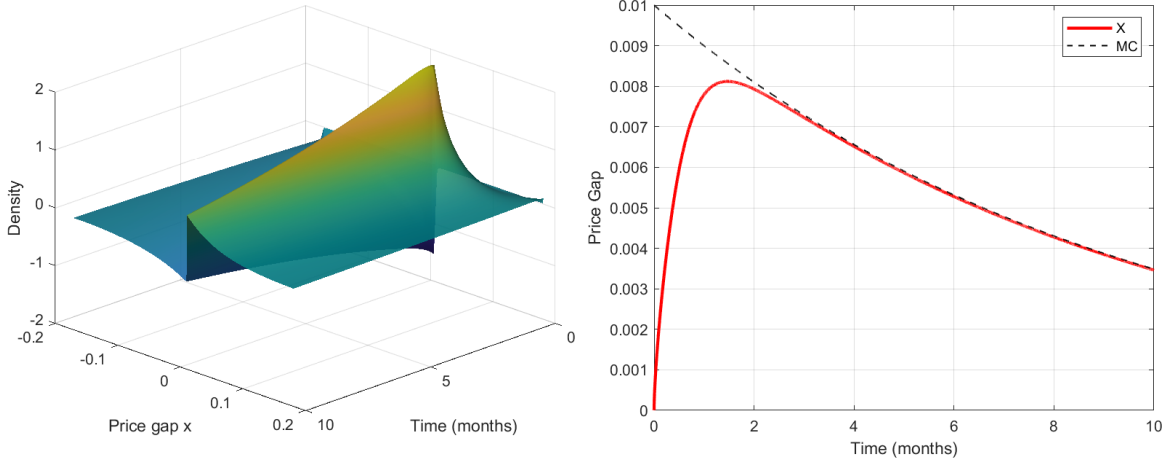
Notes: The left panel plots the distribution perturbation \hat{h}(x, t) after a marginal cost shock. The right panel plots the aggregate price gap response \hat{X}(t) and the exogenous marginal cost path MC(t) .
