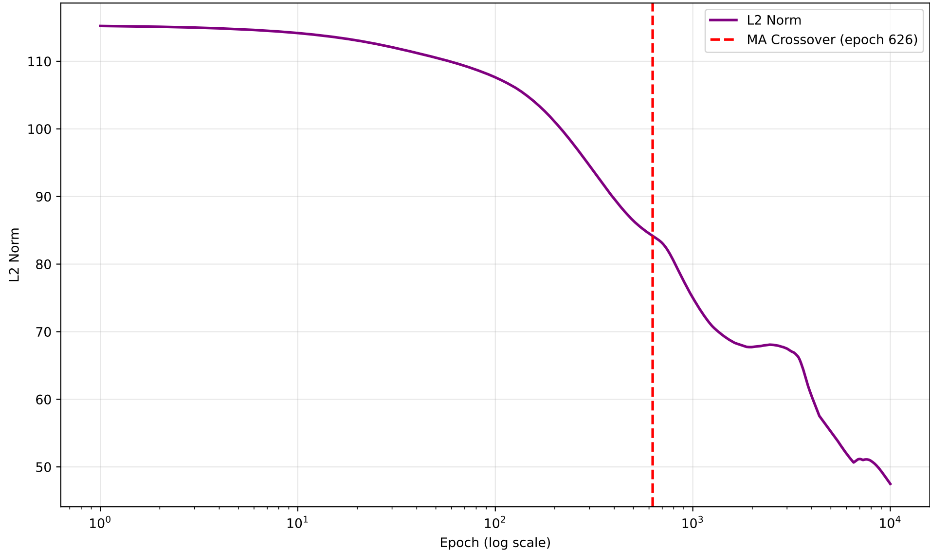
L2 Norm of Model Weights
