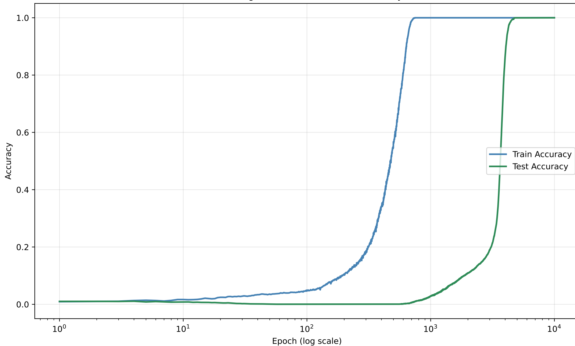
Grokking Curve: Train vs. Test Accuracy
