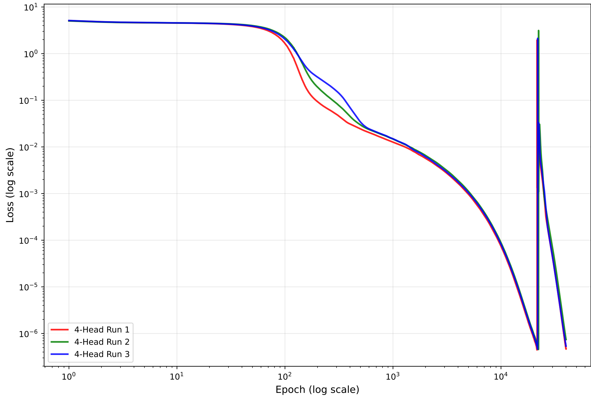
Four-Head Loss Curves
