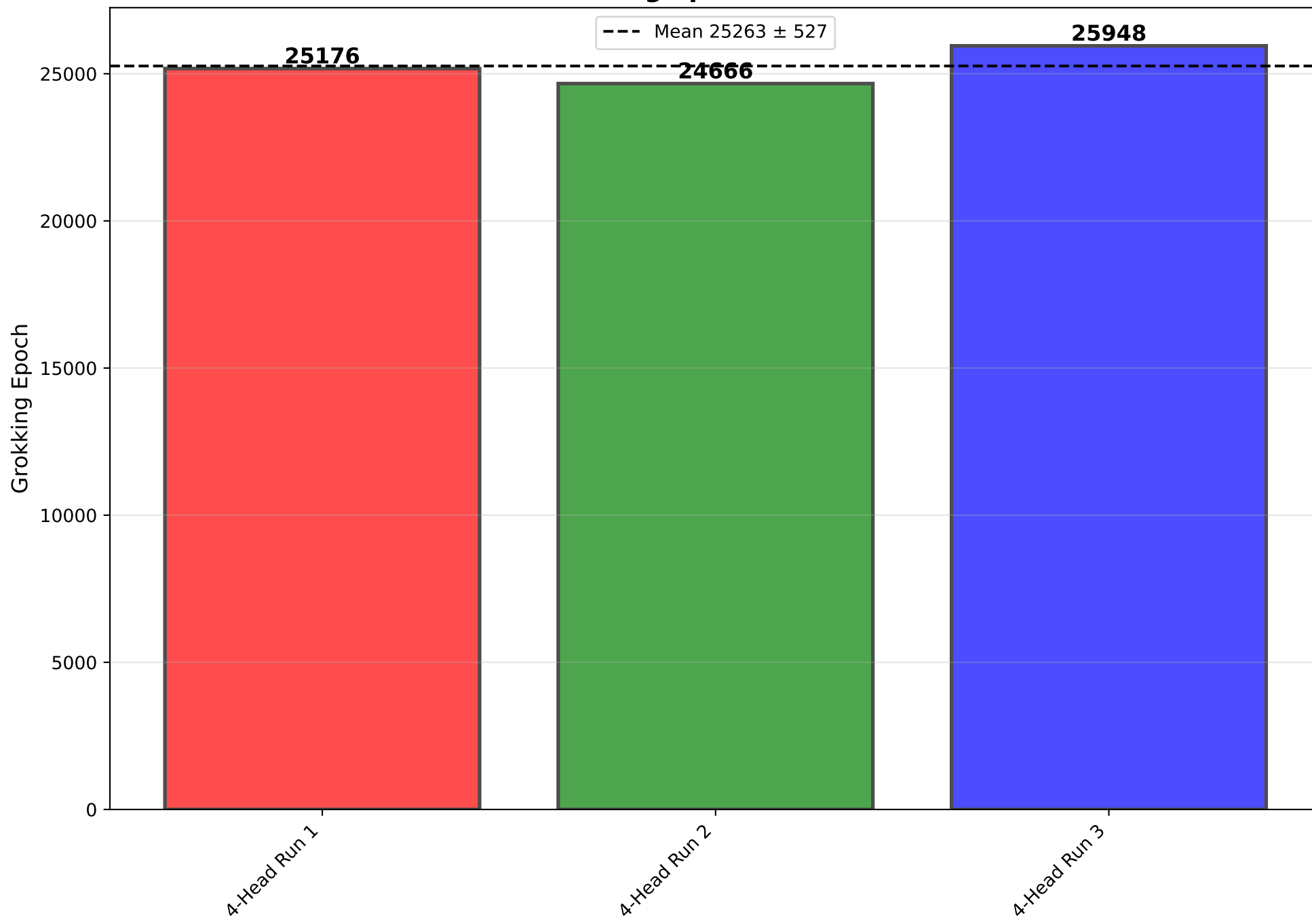
Four-Head Grokking Epoch Across Seeded Runs
